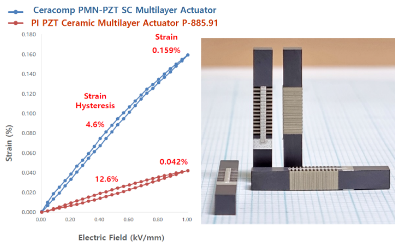
Fig. 3. Strain and strain hysteresis of two multilayer actuators: Polycrystalline PZT ceramics vs. single crystals
