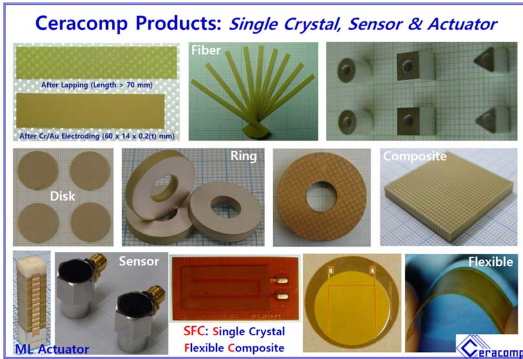
Fig. 2. "Gen III" piezoelectric PMN-PZT single crystals, single crystal-epoxy composites, SFC (Single crystal Flexible Composite), sensors and actuators
