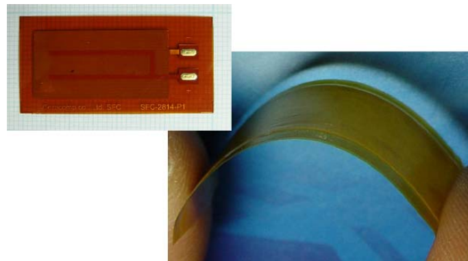
Fig. 4. "Flexible" SFC (Single Crystal Fiber Composite) for SHM
