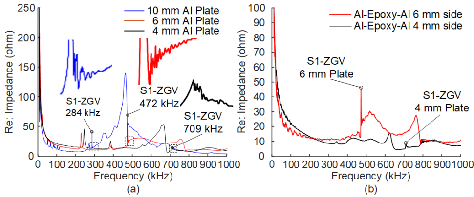
Figure 8: (a) EMI spectra of single-layer Al plates; (b) EMI spectrum of the Al-Epoxy-Al plate.
